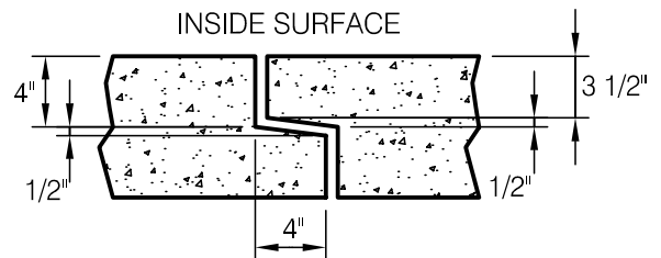
TYPICAL JOINT DETAIL
