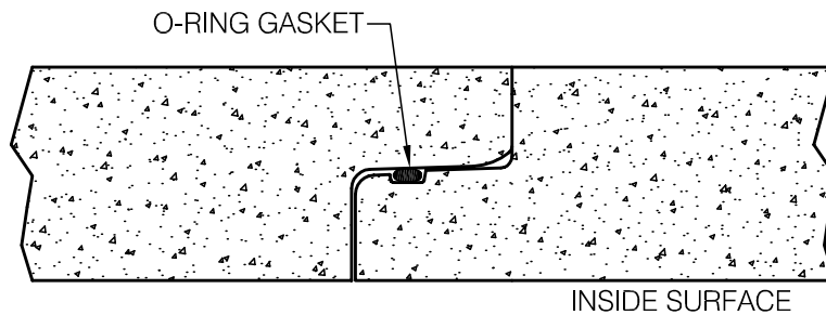
RUBBER GASKET PER ASTM C-443
