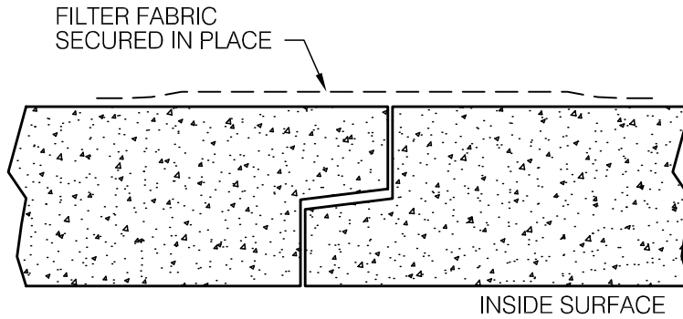
GEOTEXTILE FABRIC PER AASHTO M-288, TYPE II
