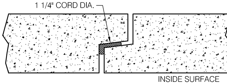
PREFORMED PLASTIC JOINT SEALANT PER ASTM C-990
