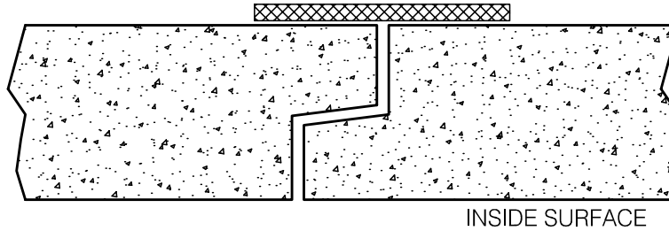
EXTERNAL JOINT SEAL PER ASTM C-877
